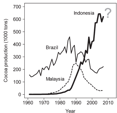
Fig. 3. Exponential growth and stagnation of cocoa production in Indonesia against the boom and bust cycles in Brazil and Malaysia: will Indonesia witness the next cacao bust? Data from FAOSTAT (2009), partly adapted from Clough, Faust & Tschardt (2009b).
